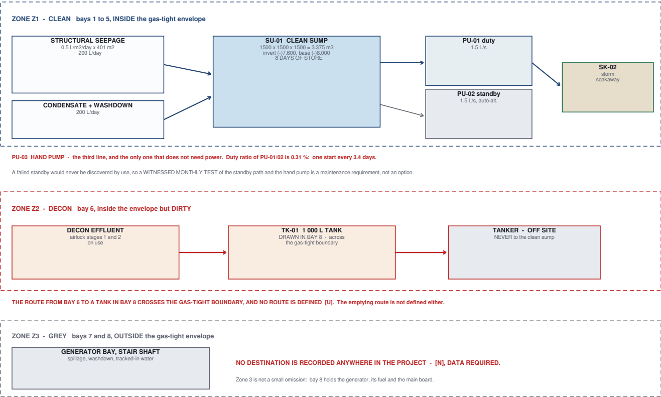
Figure 41 The three hydraulic zones, and the one that has nowhere to go.
