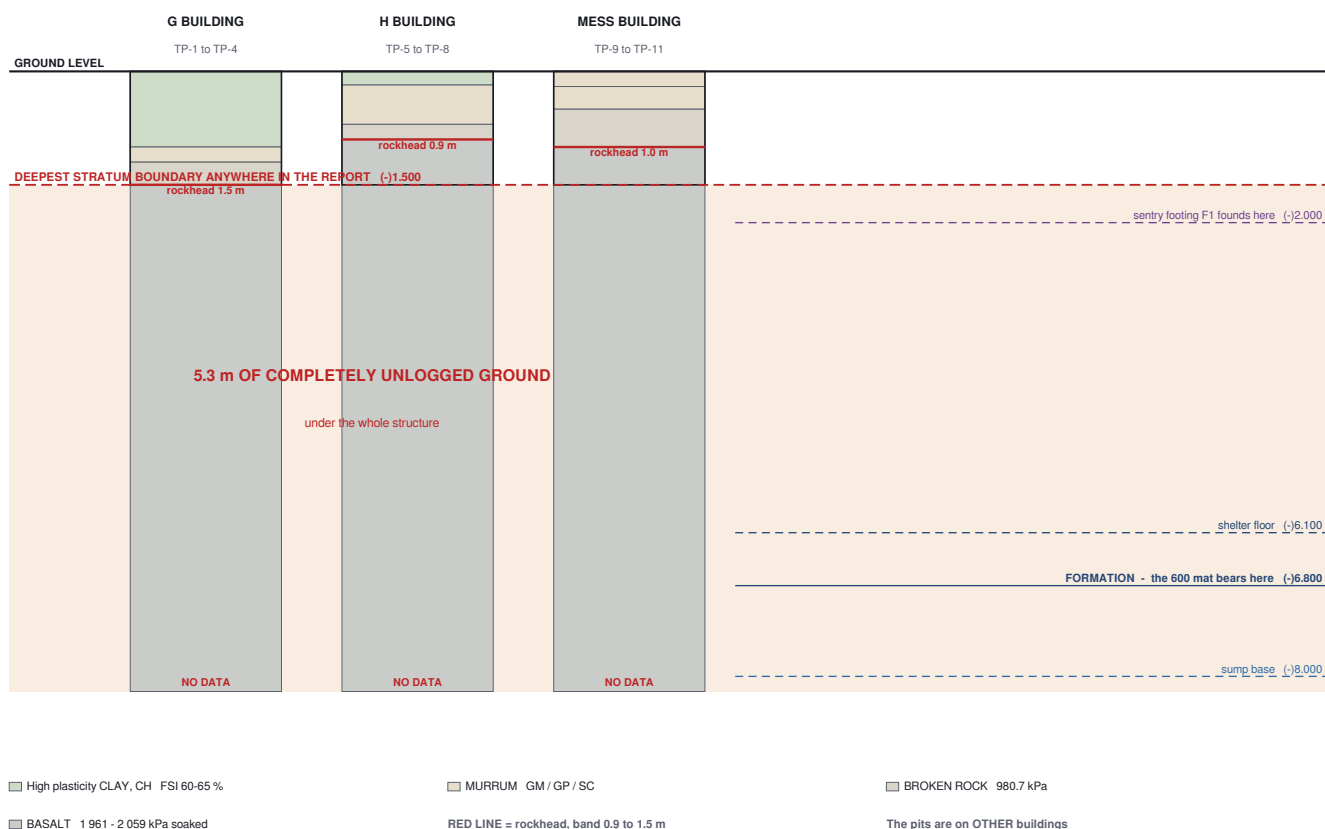
Figure 12 The sub-soil investigation against the structure it has to support. Eleven trial pits on three OTHER buildings, none deeper than 1.5 m, against a formation at (-)6.800.
