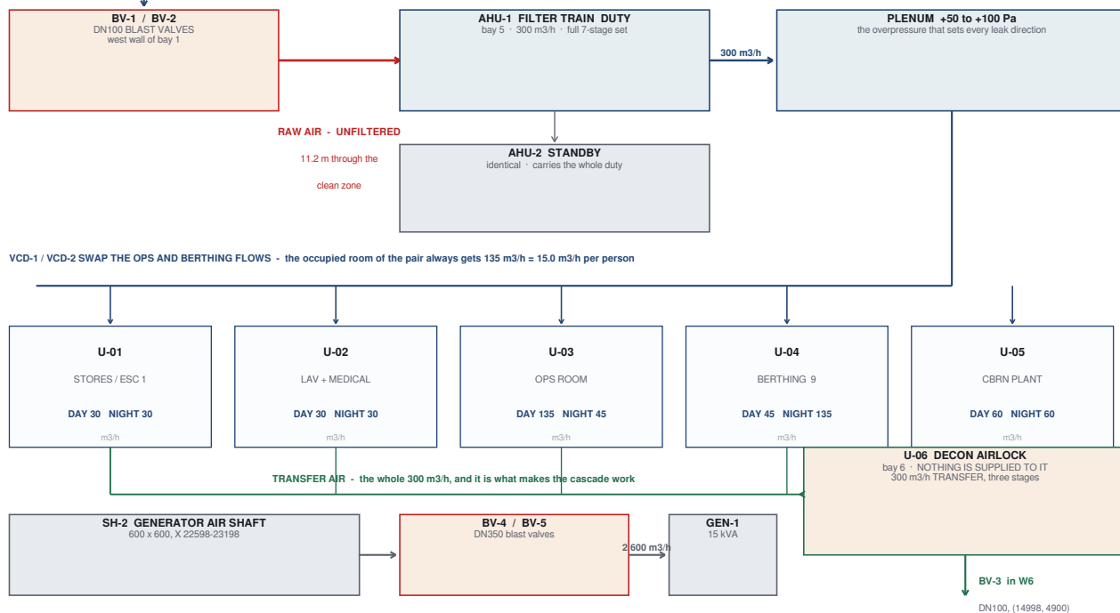
Figure 36 The whole air path - intake, the two trains, distribution, the cascade, the exhaust, and the separate generator loop.
