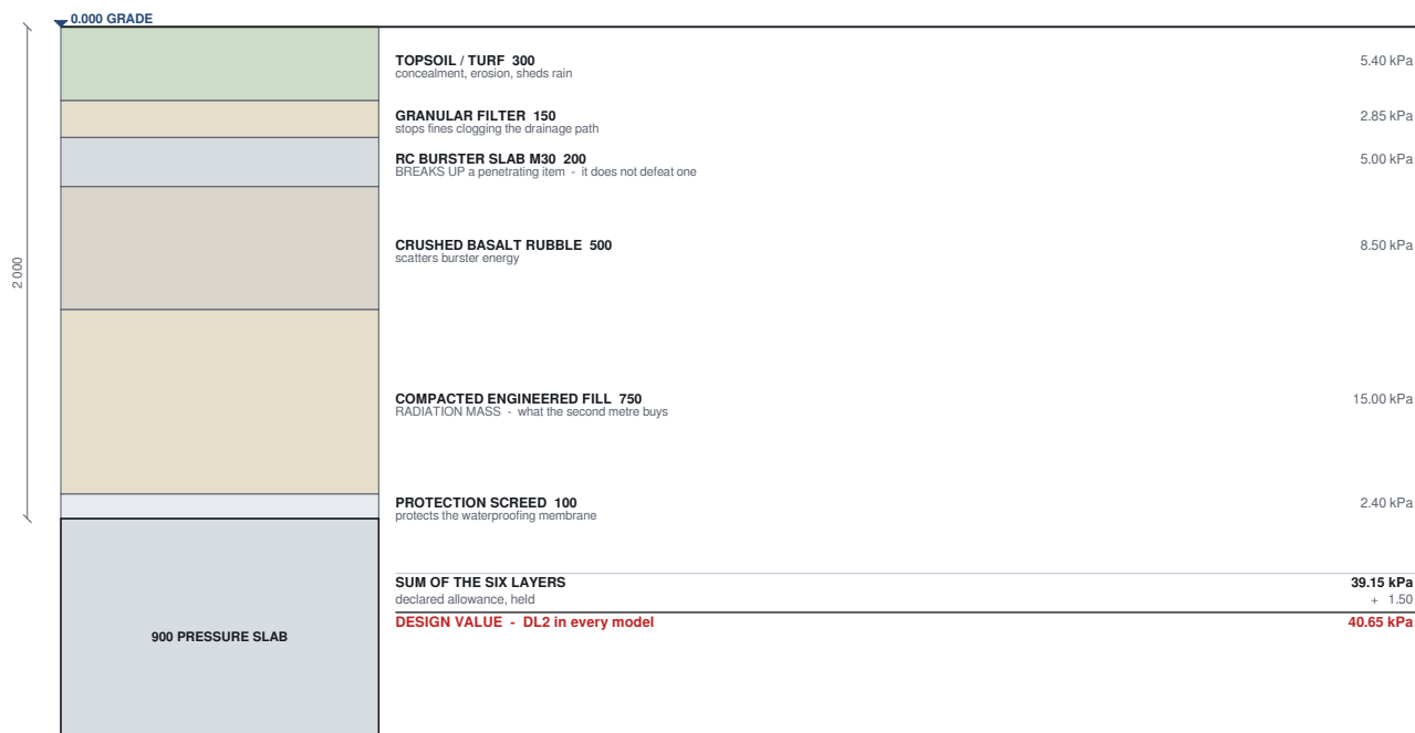
Figure 23 The engineered cover, layer by layer: 2 000 mm and 40.65 kPa.
