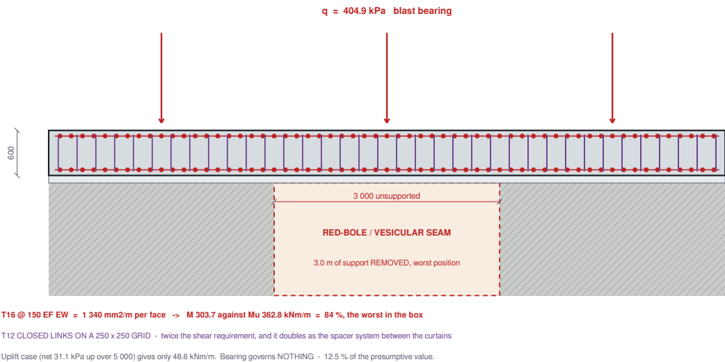
Figure 27 The mat foundation, 600 thick, and the soft-band case that sizes it.
