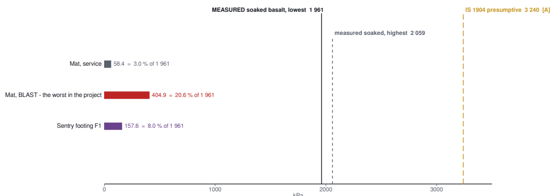
Figure 13 Bearing demand against capacity. The worst case in the project uses 20.6 per cent of the lowest measured soaked strength.
