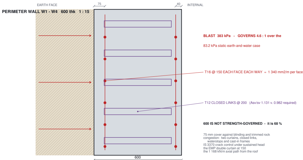
Figure 25 Perimeter wall W1 to W4, 600 thick - section and reinforcement.
