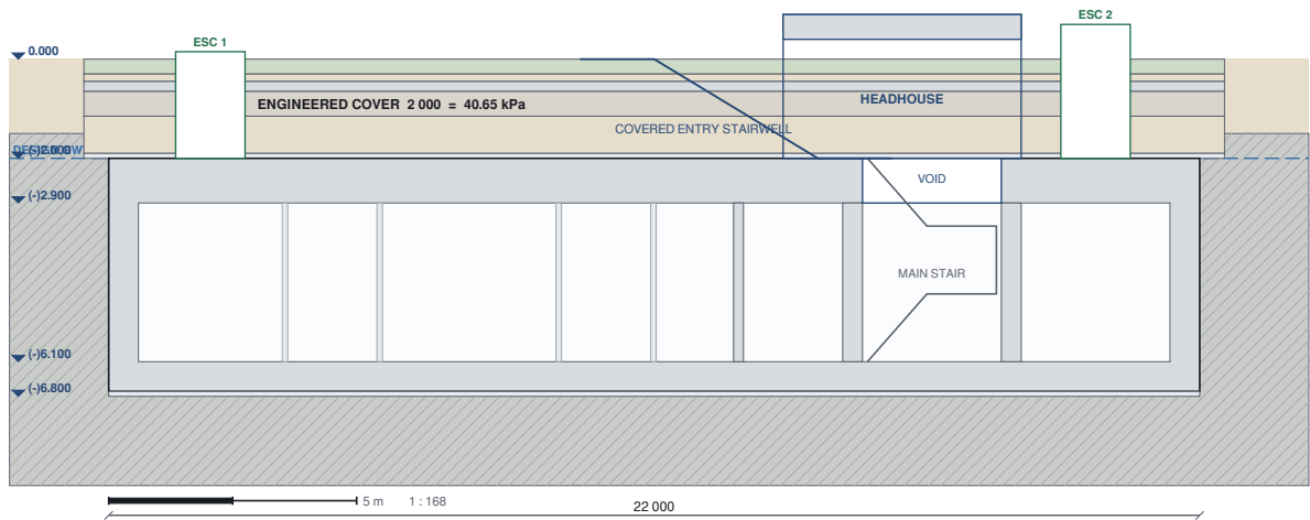
Figure 17 Longitudinal section on the spine, from the west end to the generator bay.
