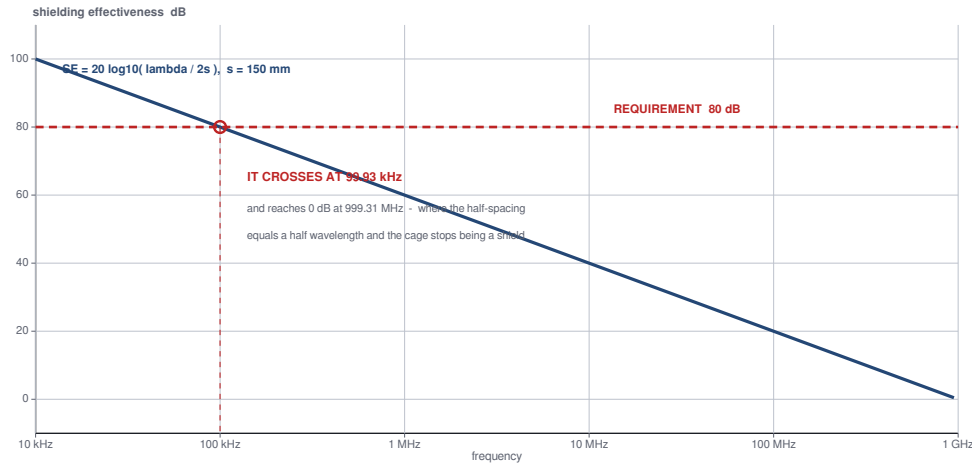
SHIELDING EFFECTIVENESS OF THE REINFORCEMENT CAGE - 20 dB PER DECADE AGAINST A FLAT 80 dB REQUIREMENT
