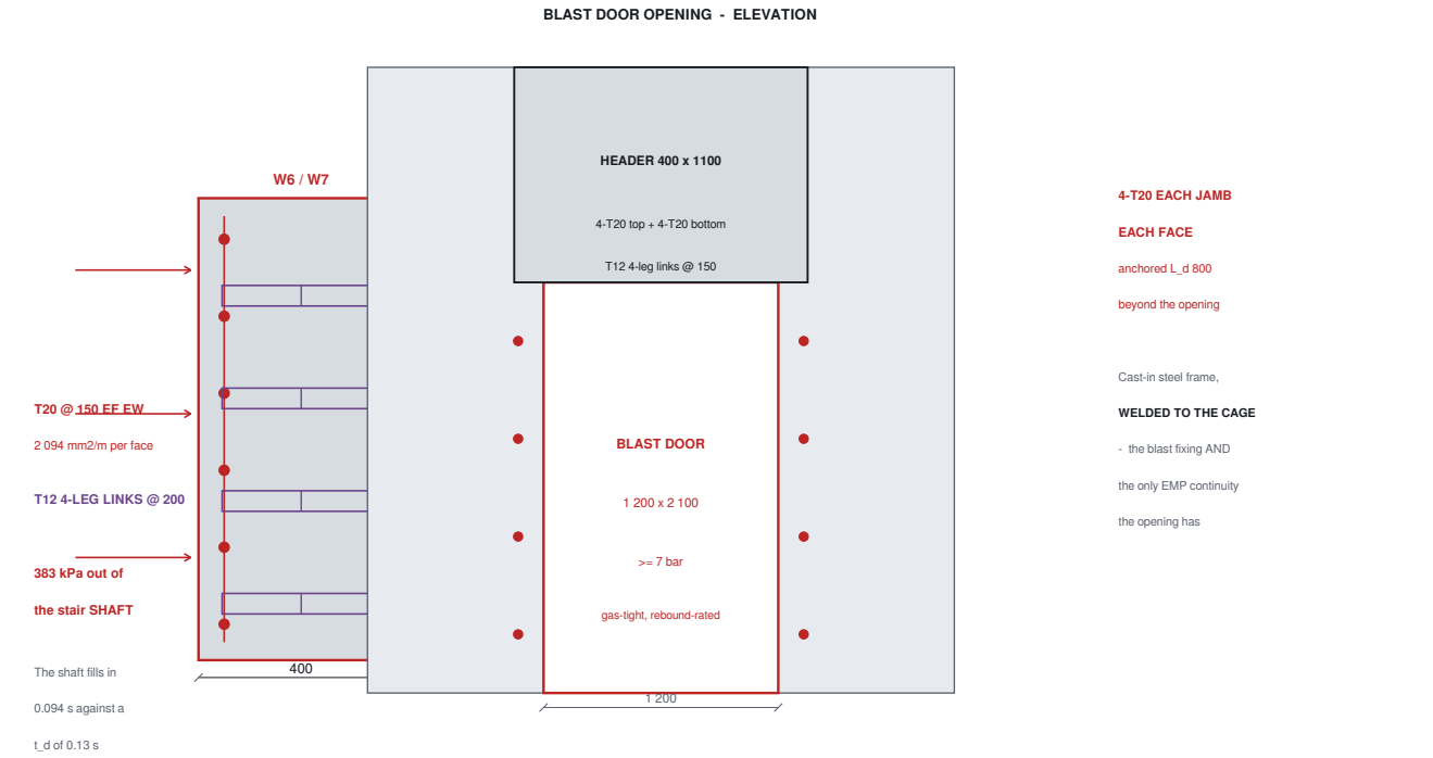
Figure 26 Walls W6 and W7 at 400, and the blast door openings they carry.
