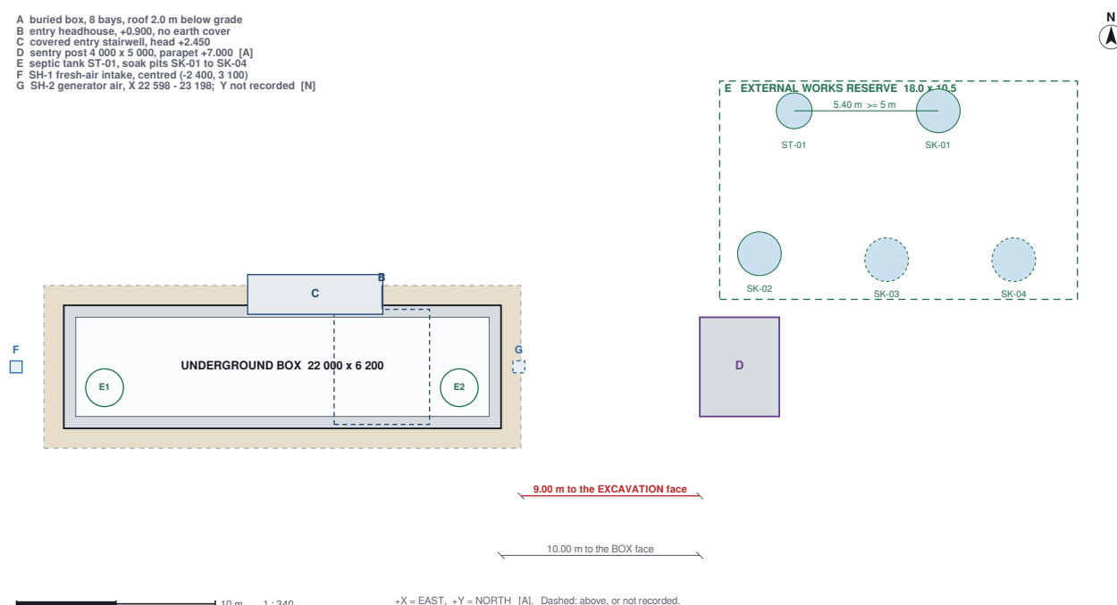
Figure 11 Key plan. Everything on the plot at true project coordinates - the buried box, the headhouse, the covered entry stairwell, the two escape shafts, the sentry post and the reserve.
