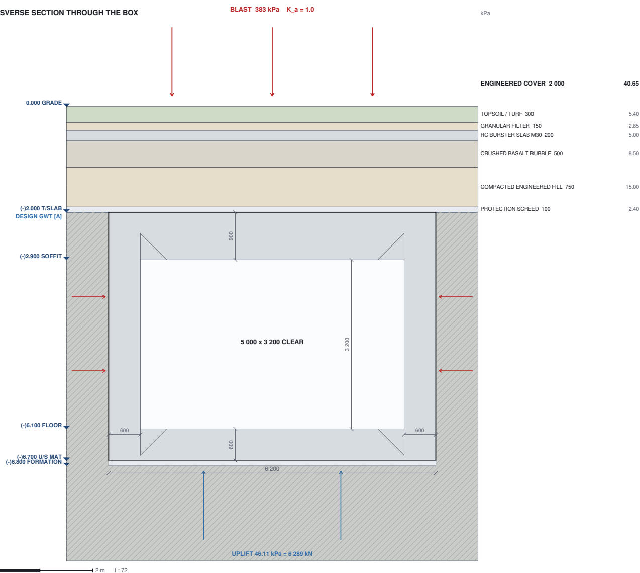
Figure 18 Transverse section through the box, with the full engineered cover build-up and the load that arrives from each direction.
