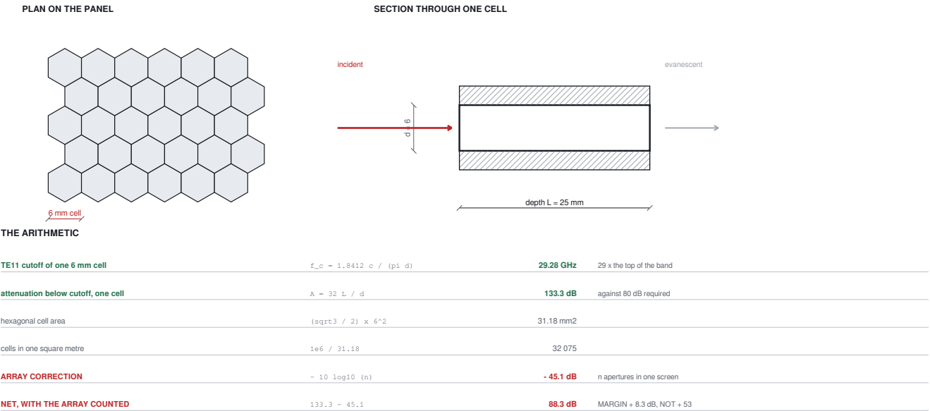
THE SINGLE-CELL NUMBER IS AN UPPER BOUND, AND THE ARRAY CORRECTION IS WHY VENDOR TEST DATA IS NOT OPTIONAL. A panel still passes at 88 dB, but a margin of 8 dB is a margin a bad gasket eats. Mount the panel INBOARD of the blast device - the valve takes the pressure, the honeycomb takes the radio frequency - and require a certified attenuation curve for the panel as built, not for one cell. Two consequences are referred rather than resolved: a honeycomb panel adds pressure drop, and the fan duty was built without one; and the panel's own blast rating is [N].
