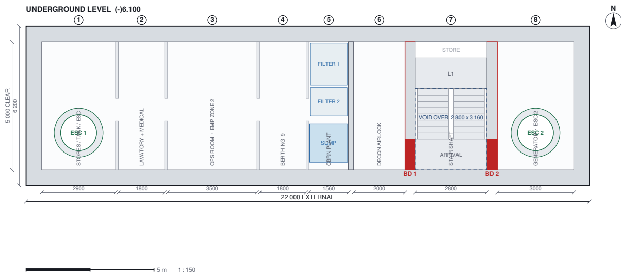
Figure 16 The underground box in plan - eight bays, the two escape shafts, the stair shaft and every internal wall.
