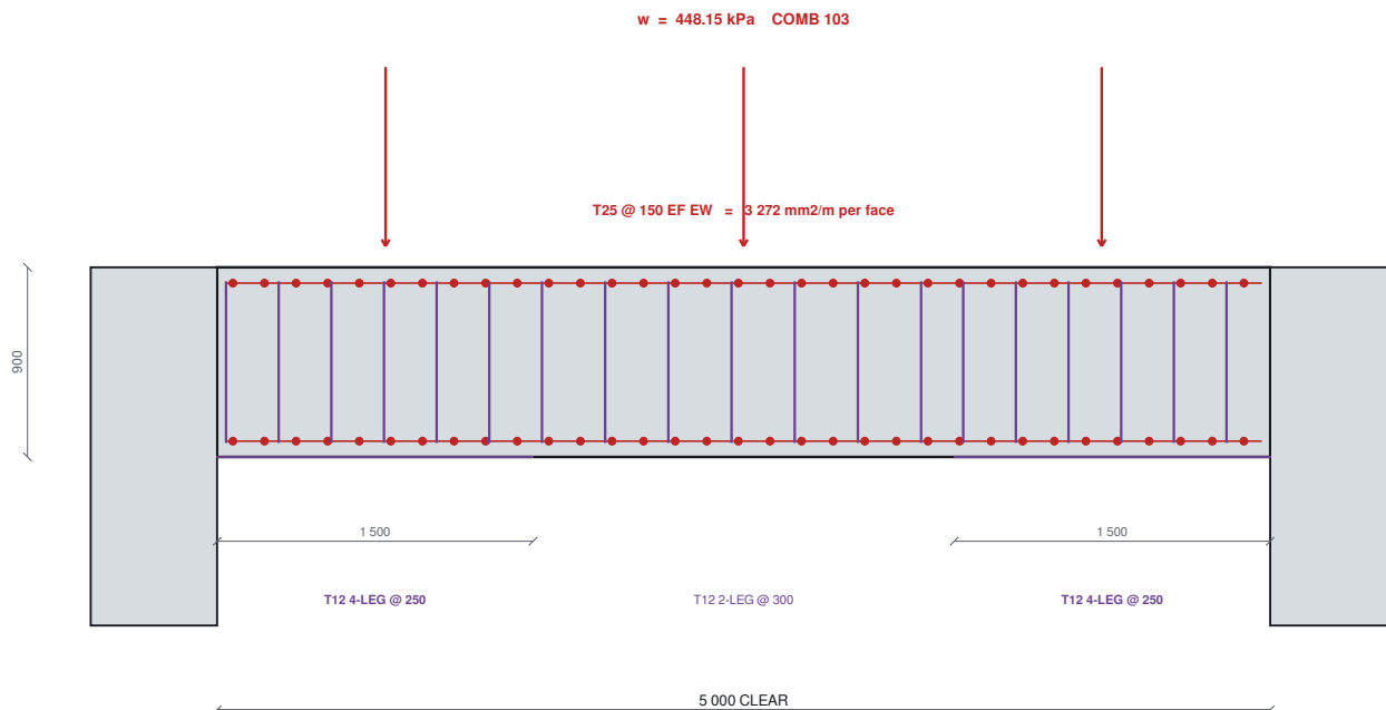
Figure 29 The pressure slab, 900 thick - the governing element.
